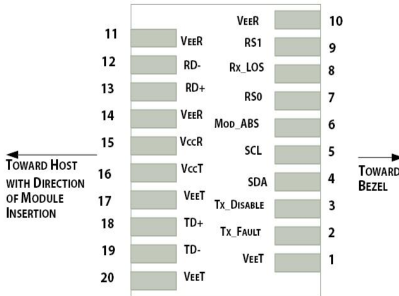
Figure1.Electrical Pin-out Details
