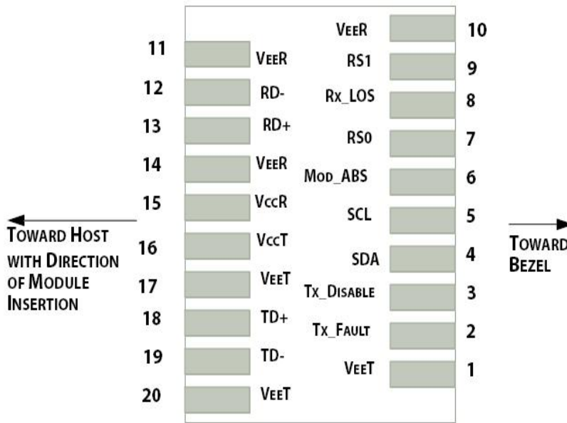
Figure1.Electrical Pin-out Details
